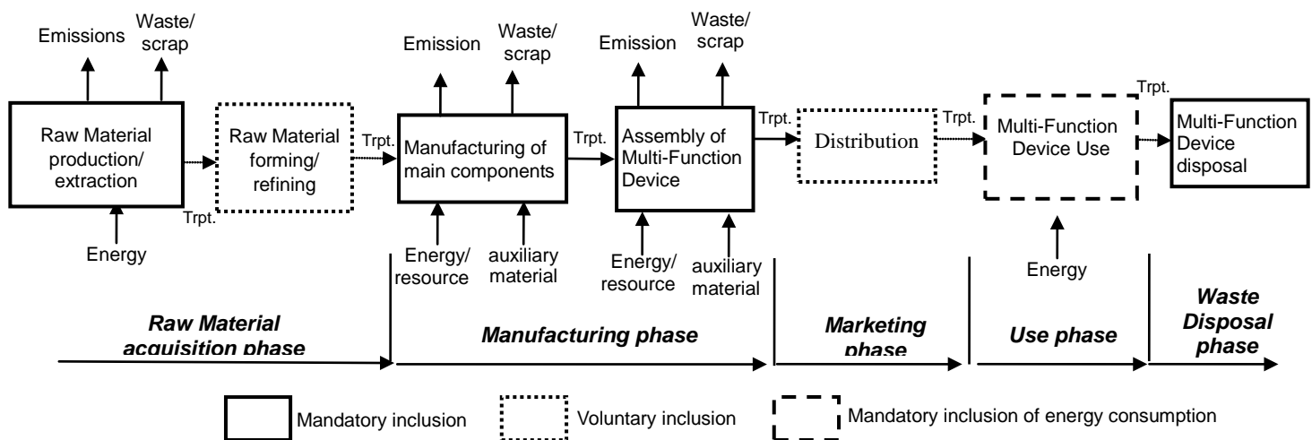
Figure 1 System boundary of the product system
