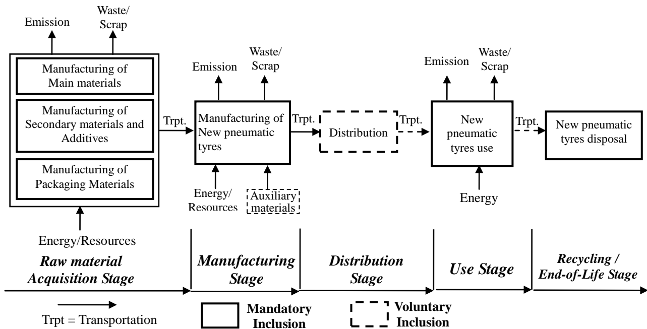
Figure 1 System boundary of the product system
