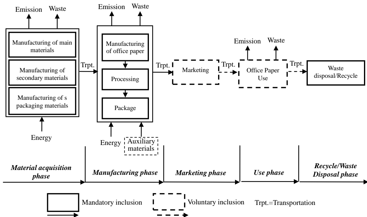
Figure 1 System boundary of the product system
